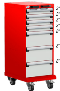
7 tiroirs L3BBD-4009 18" x 21" x 45 1/8" L3BBG-4009 18" x 27" x 45 1/8"
